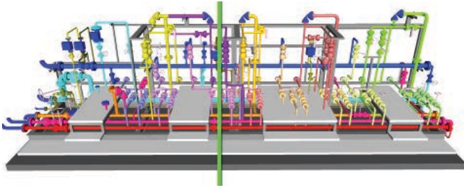
A plan for how the flange connection units were to be divided.
